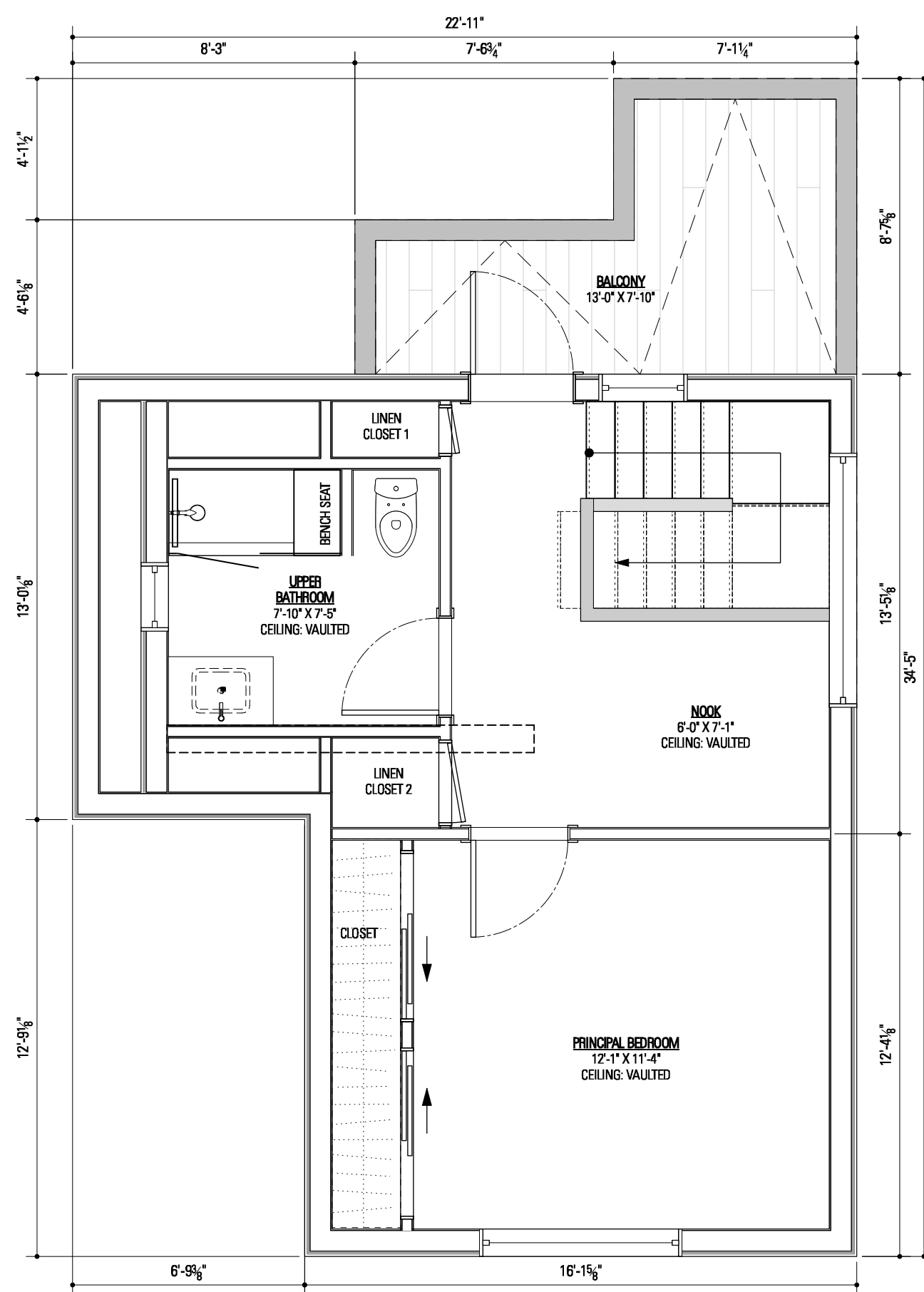
2 UPPER FLOOR
