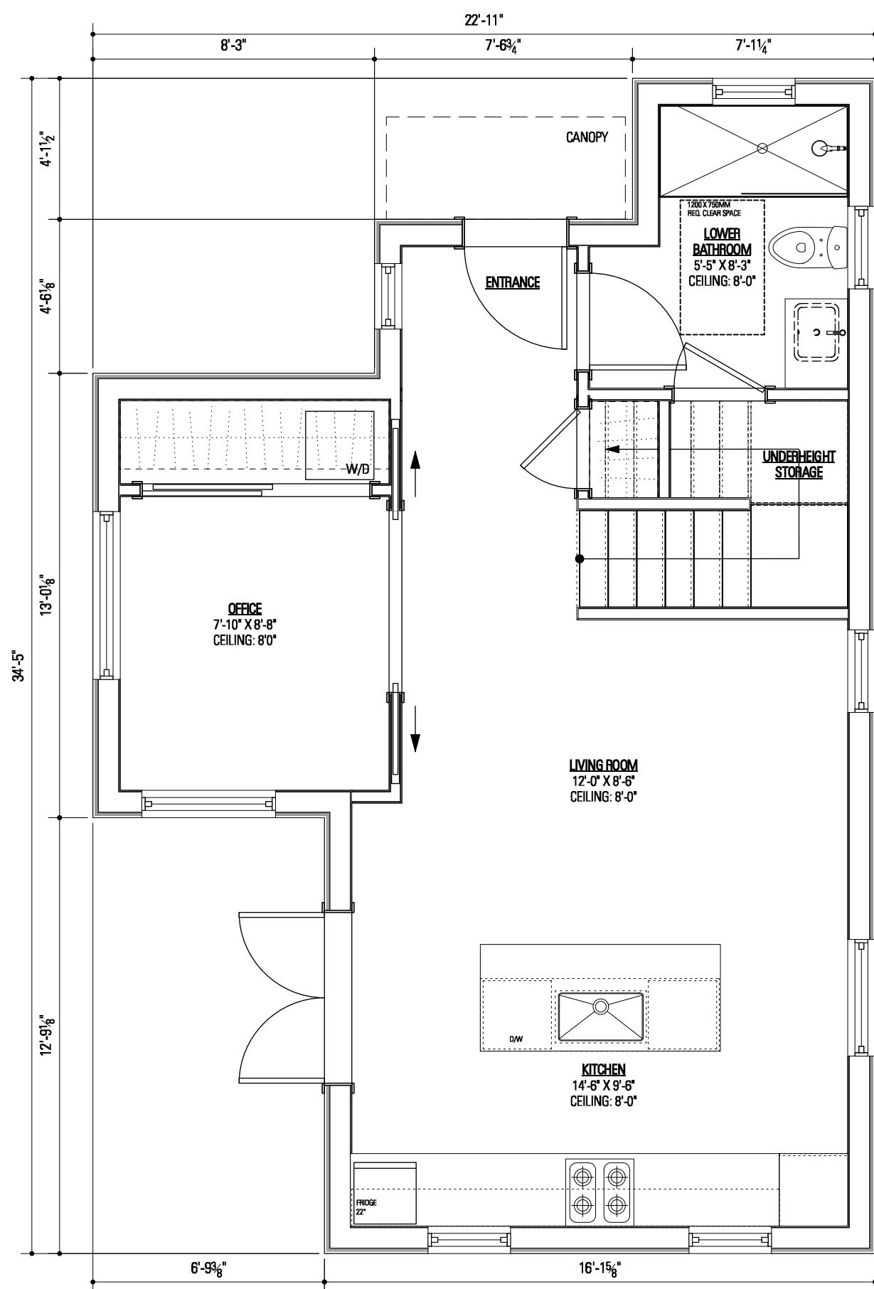
1 MAIN FLOOR
